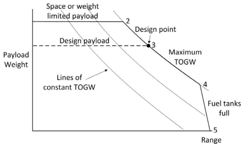
Figure 15.1 Payload-range Plot
