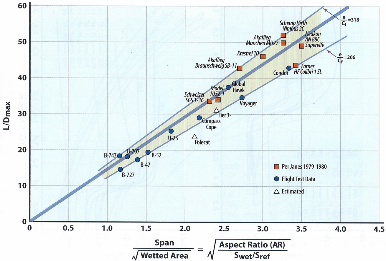
Fig. G.8 Max. L/D Correlation Curve—Flight Test Data
