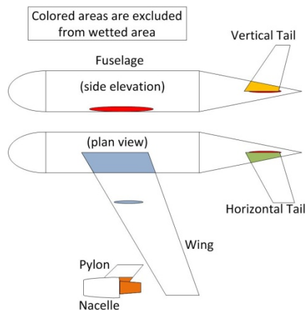
Figure 12.2 Wetted area buildup
