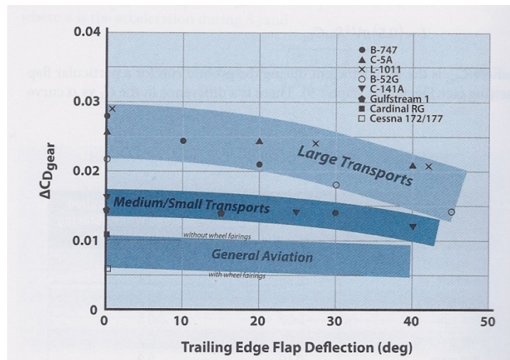
Figure 12.4 Parasite Drag Increment due to Landing Gear Extension
