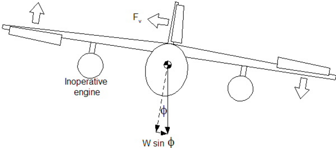
Fig. 16.4.1 Lateral forces in engine-out operation
